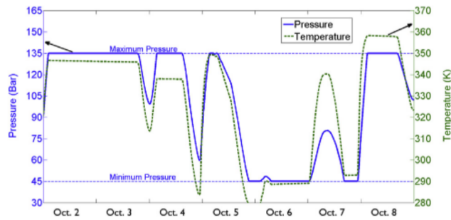
Fig. 6 – Variations of pressure and temperature inside the carven in compressed air energy storage system.
