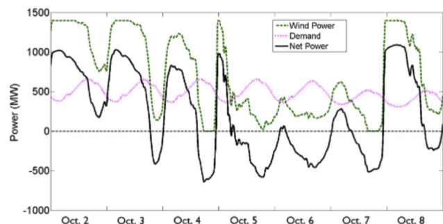
Fig. 5 – Power profiles of wind, demand and net power, October 2006.
