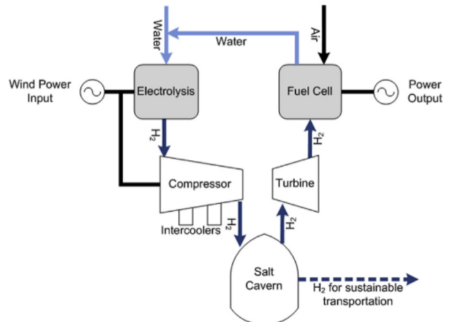
Fig. 2 – Schematic of compressed hydrogen energy storage system.
