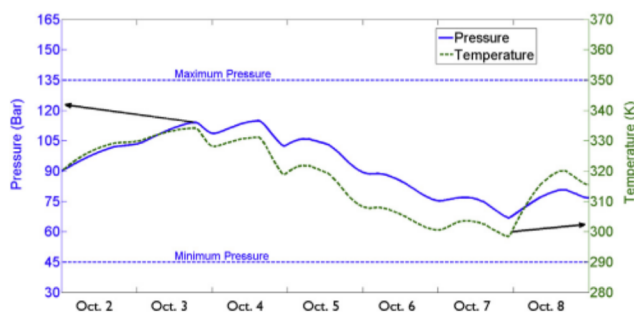
Fig. 7 – Variations of pressure and temperature inside the carven for the compressed hydrogen energy storage system.
